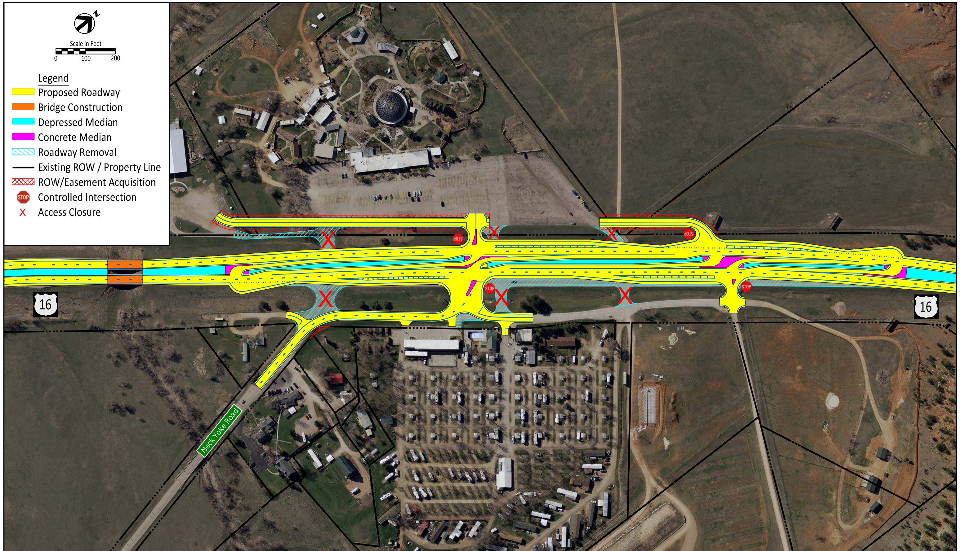
Neck Yoke Road Reduced Conflict Intersection (RCI) - Central Driveway with US16 Realignment US16 Corridor Study
