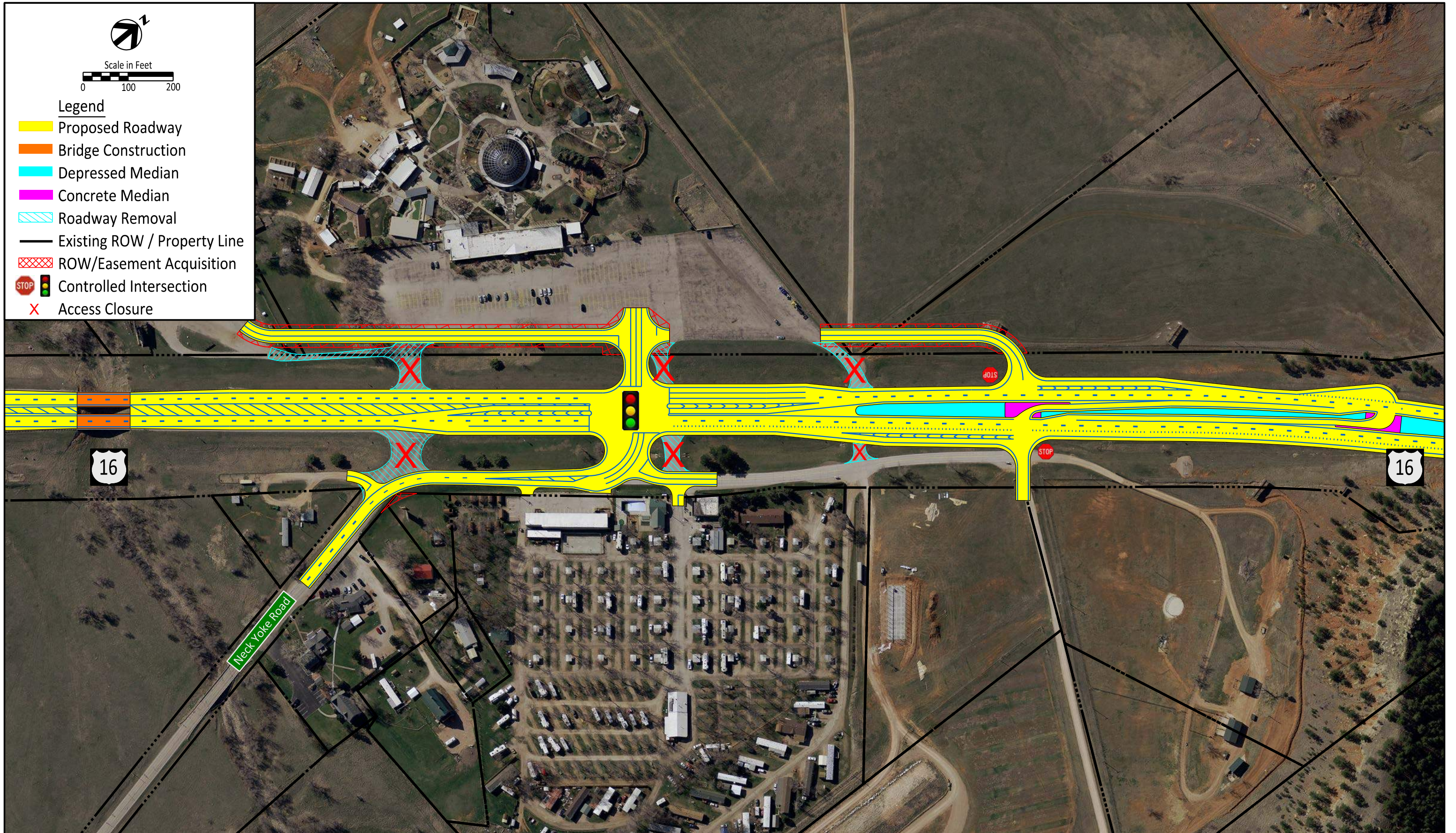
Neck Yoke Road Signalized Intersection - Central Driveway US16 Corridor Study
